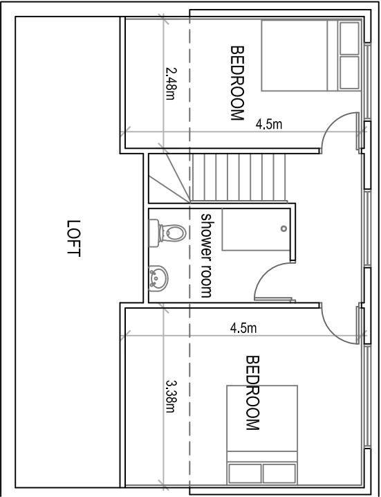
PROPOSED SF PLAN 1:100
